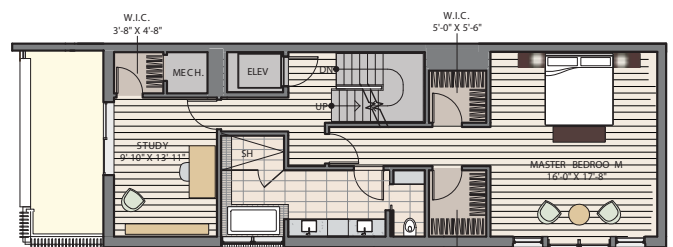
FOURTH FLOOR
