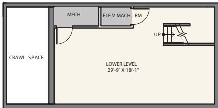
LOWER LEVEL
