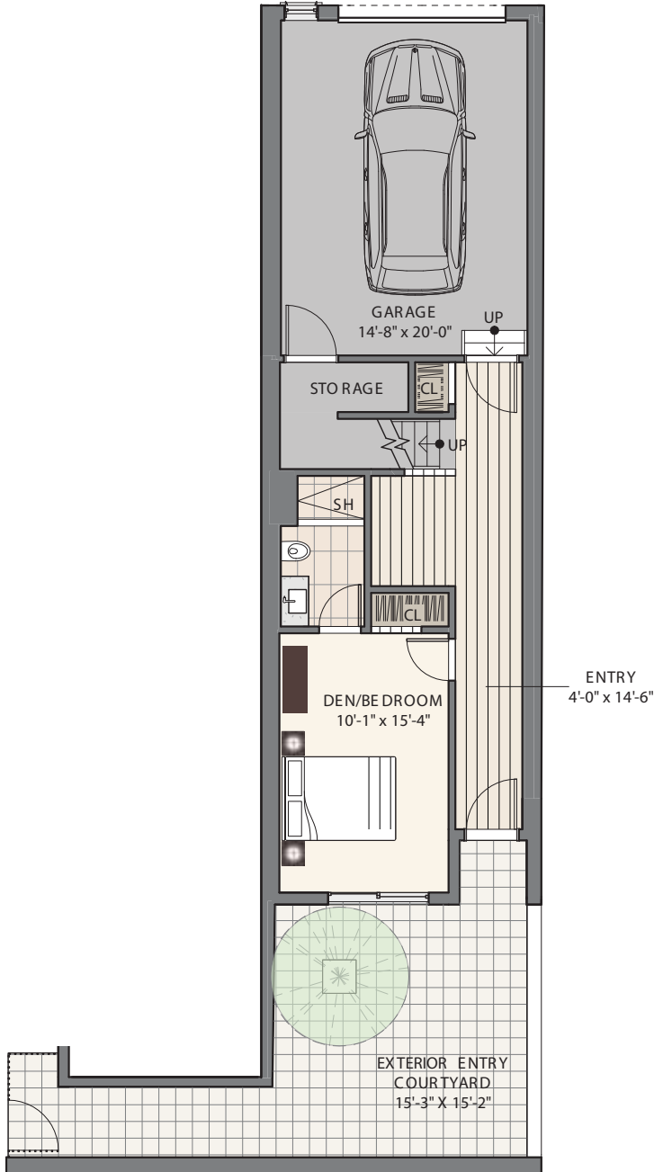
FIRST FLOOR
